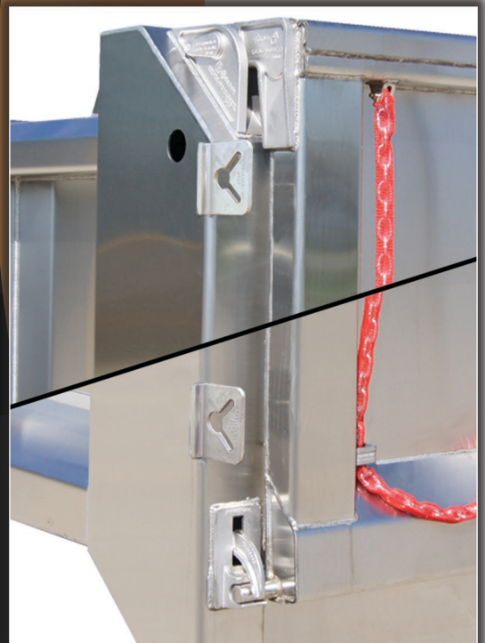
All hardware on the 403U/T is stainless to promote longevity through corrosion resistance
