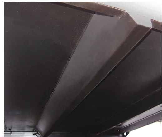
The crossmemberless understructure of the 130U & 133U Crossmemberless body uses 3/16" X 100K formed 5" trapezoidal longbeams.
