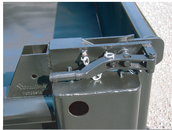
Pictured is a close view of the upper quick release hardware. This hardware makes it easy to quickly remove and reinstall the tailgate.
